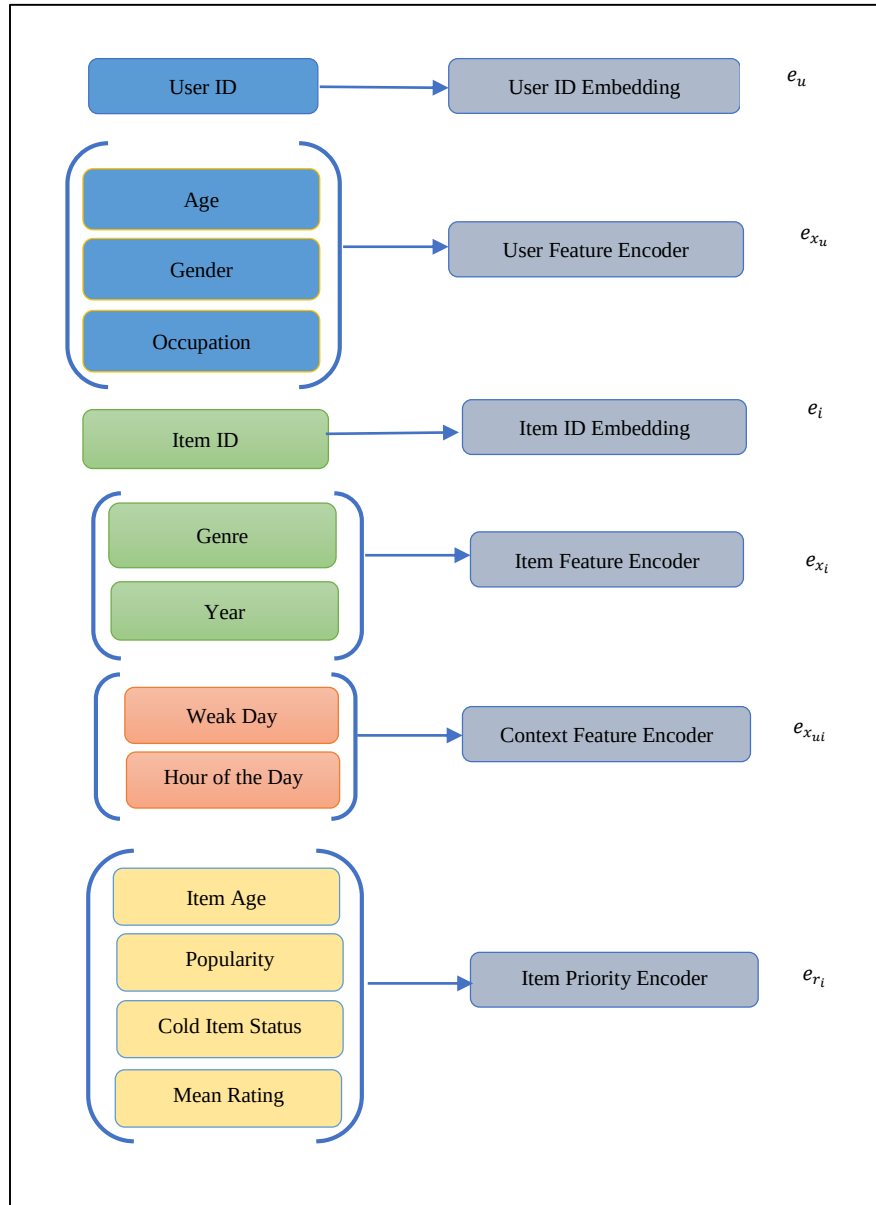
Fig. 2 Embedding representations in DeepACF
