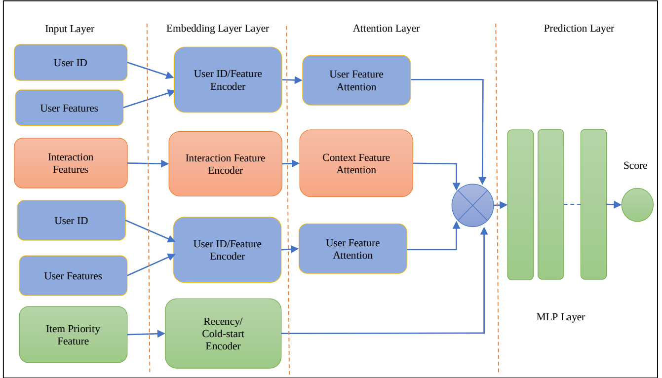
Fig. 1 Proposed architectural diagram of DeepAC
