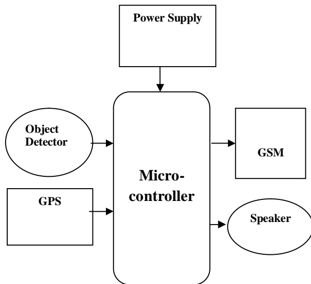
Fig 1. Proposed Smart Stick System
